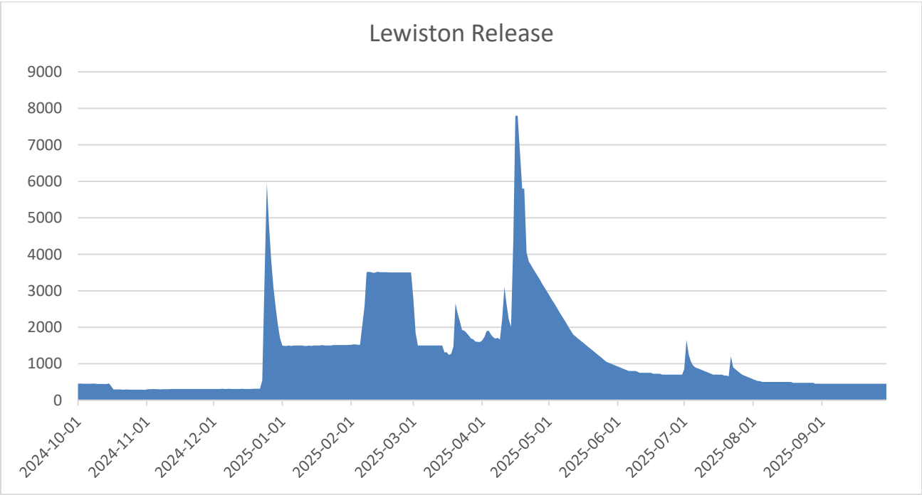
Figure 2: Normal February – Wet March – Wet April Hydrograph
