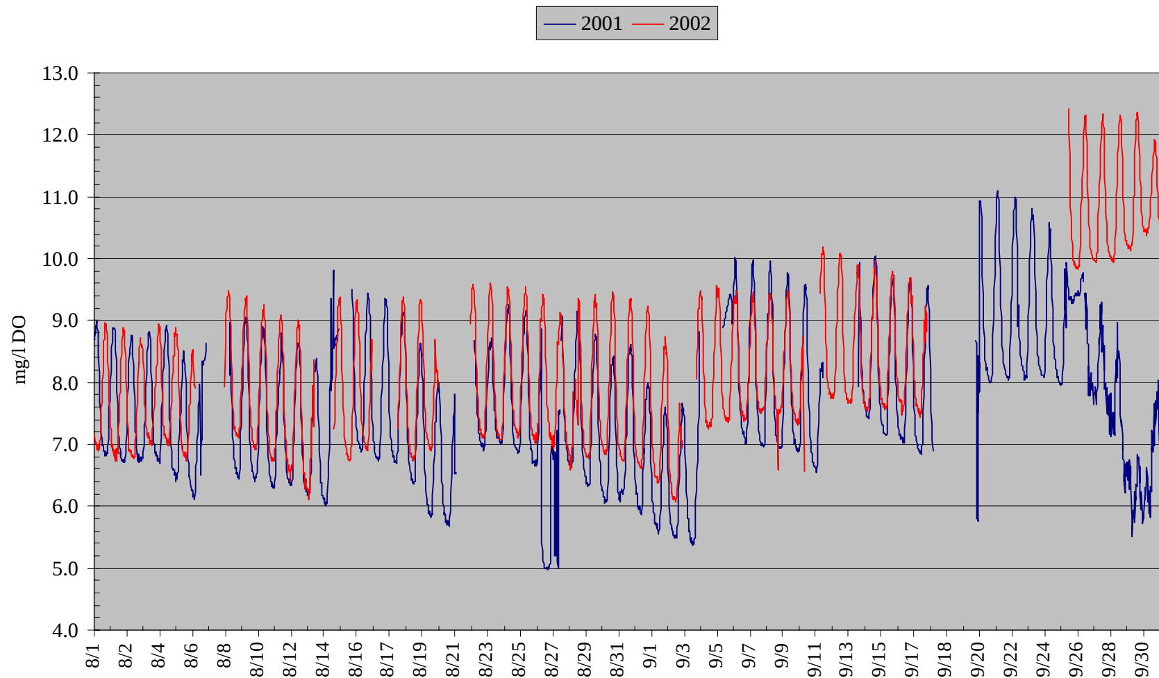
Figure E5. Dissolved oxygen concentrations for Klamath River at Weitchepc recorded at 30 minute intervals for August - September 2001 and 2002. Provisional data provided by the Yurok Tribe.
