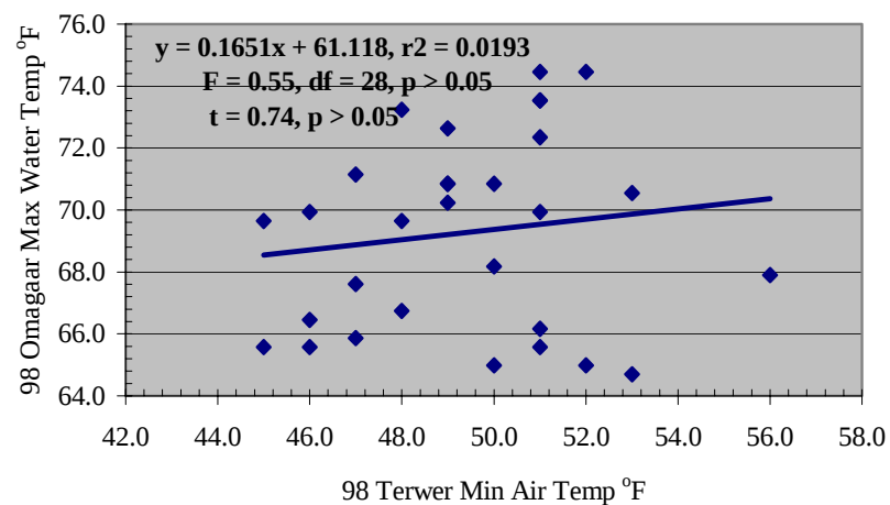
Figure D4. Regression of maximum daily September water temperatures in the lower Klamath River (1998 and 1999 at Omagaar and 2001 and 2002 at Terwer) against minimum daily air temperatures at Terwer.
