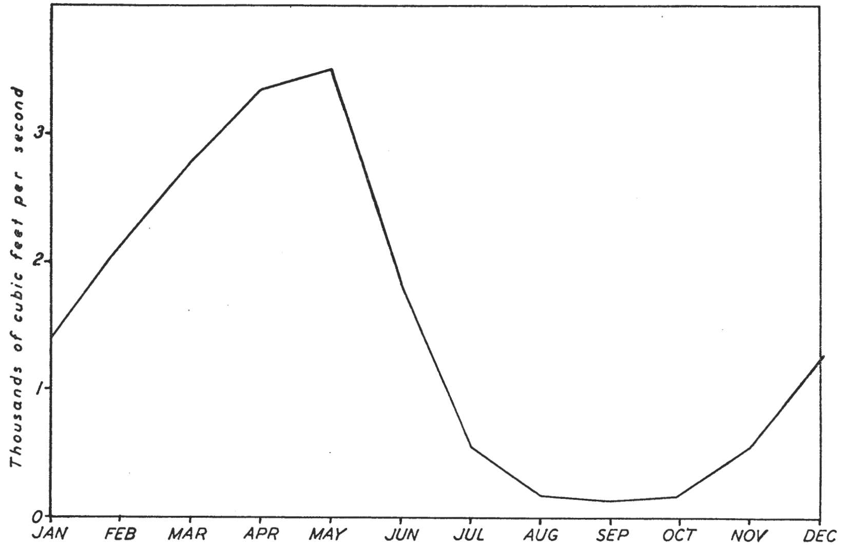
Figure 2. Average monthly flow of Trinity River at Lewiston during water years 1928-1942.
